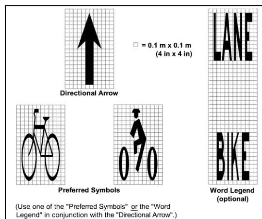
Figure: Bike Lane Pavement Markings
