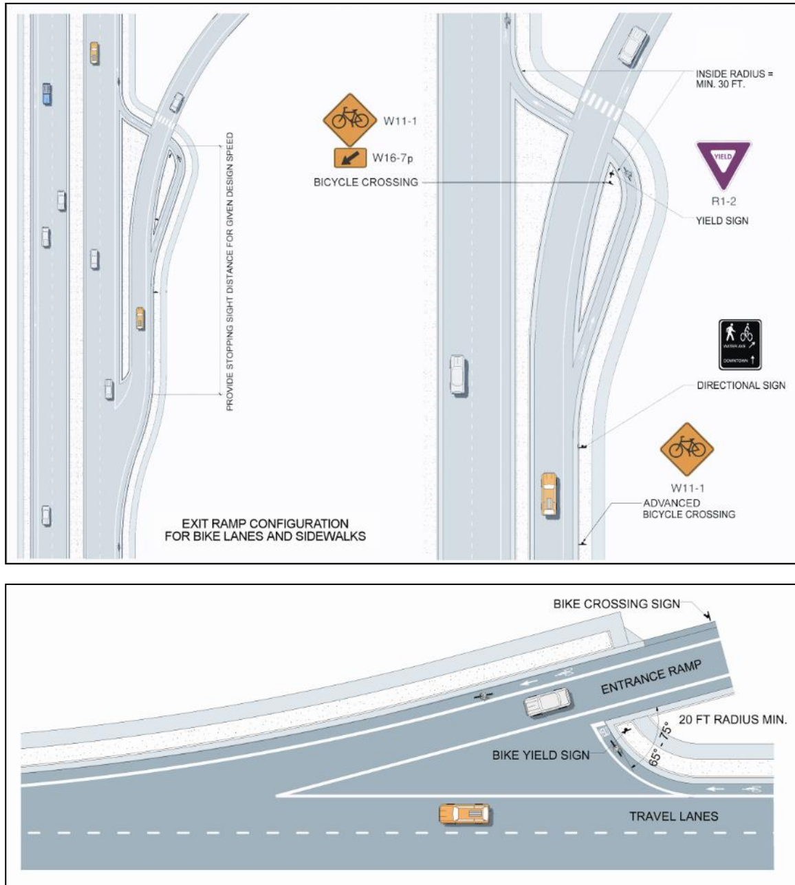
Figure: Interchanges
