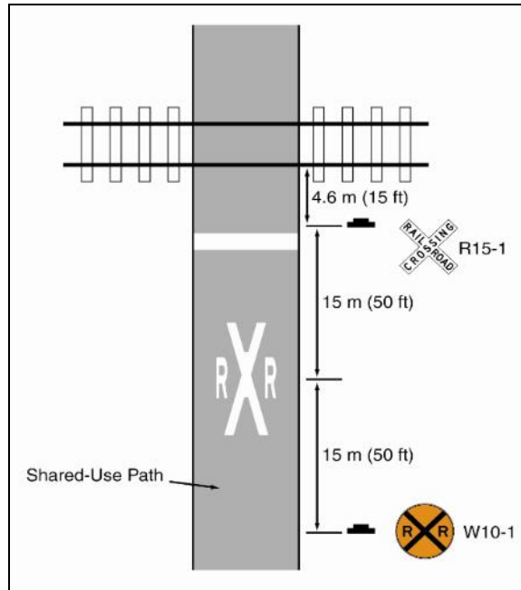
Figure: Railroad Crossing Signage
