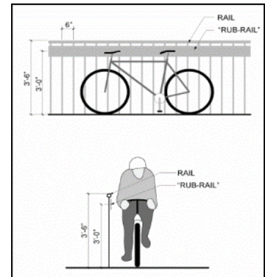
Figure: Railings and Fencing
