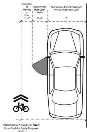
Figure: Sharrow Pavement Marking
