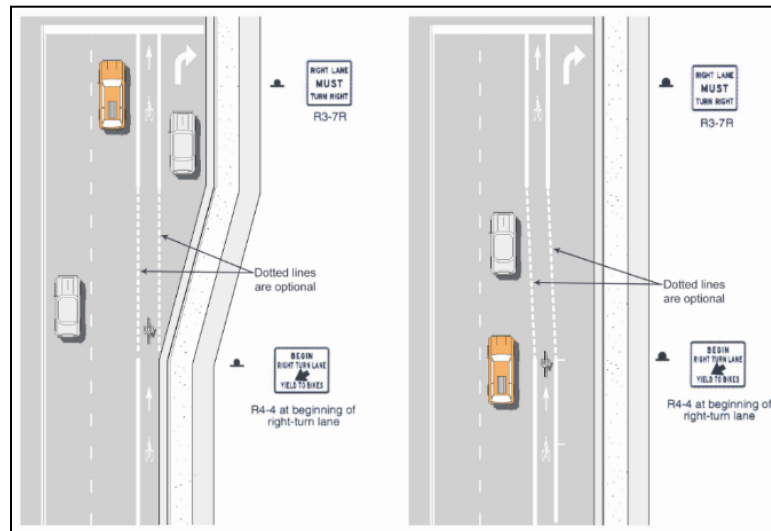
Figure: Intersection with Right-Turn Lanes
