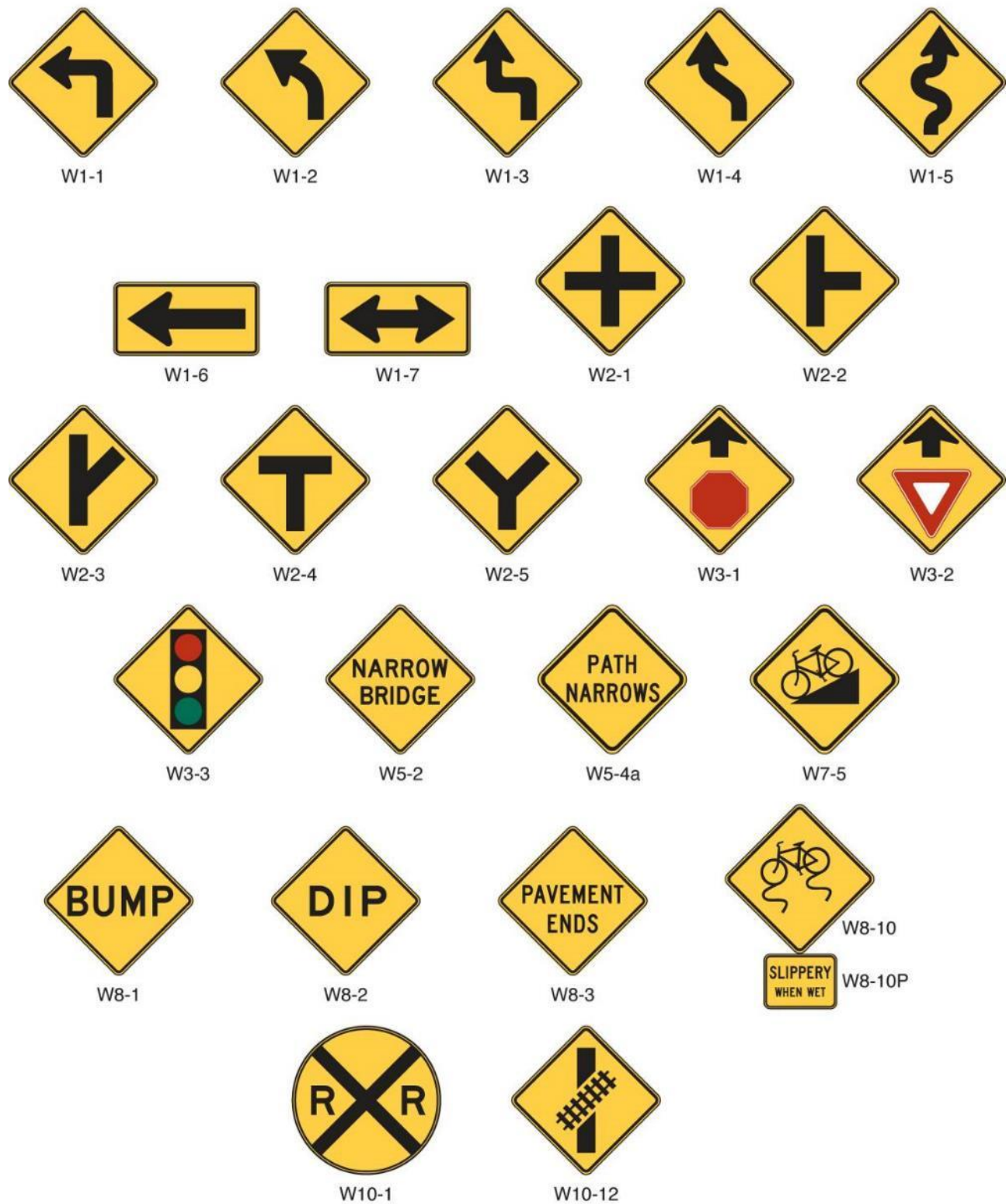
Figure (continued): Regulatory, Warning, and Directional Signage for Bicycle Facilities
