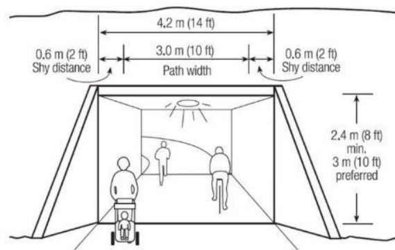
Figure: Underpass
