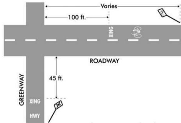
Figure: Midblock Crossing
