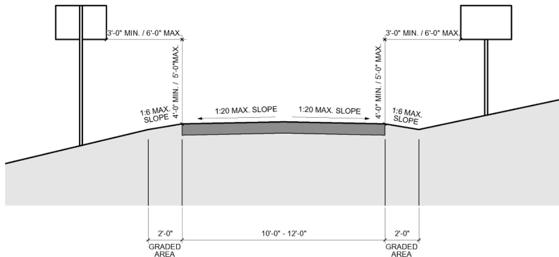
Figure: Recommended Width, Lateral Clearance and Slope Standards for Multi-Use Paths
