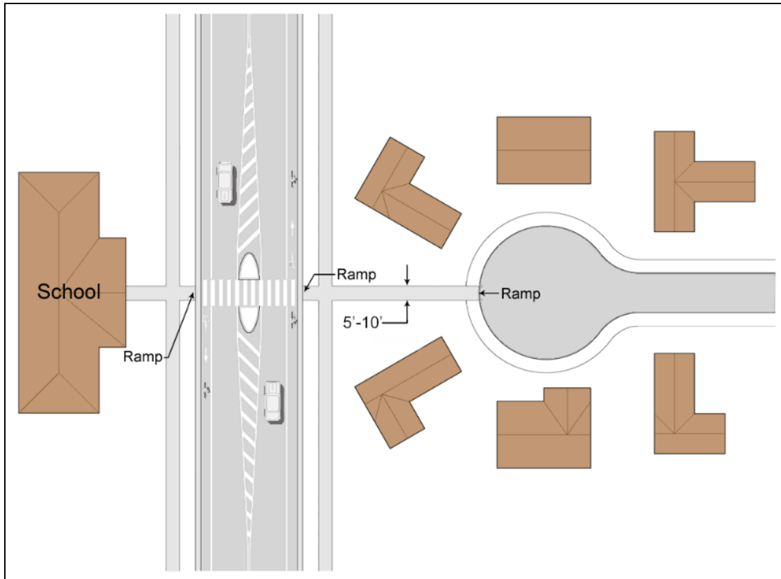
Figure: Connector Facilities
