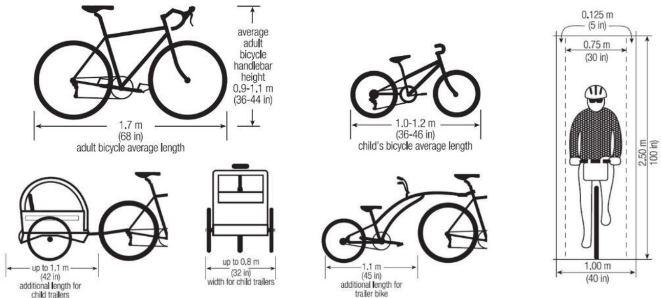
Figure: Bicyclist Dimensions
