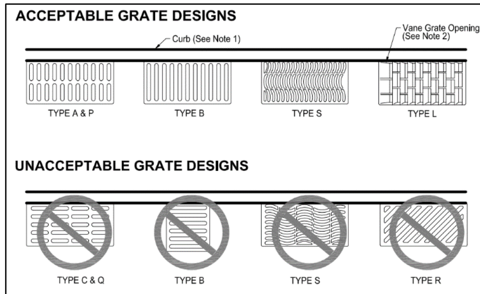
Figure: Bicycle-Friendly Storm Grate Designs
