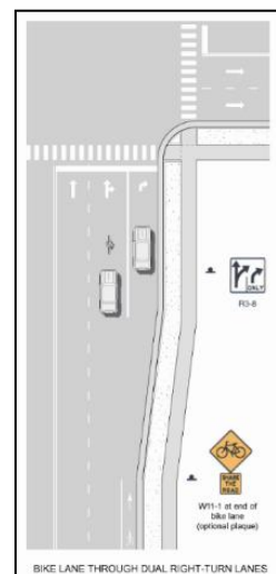
Figure: Dual Right-Turn Lanes
