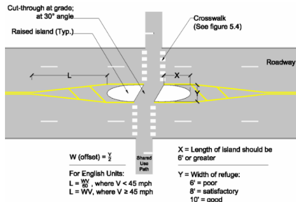
Figure: Angled Median Island
