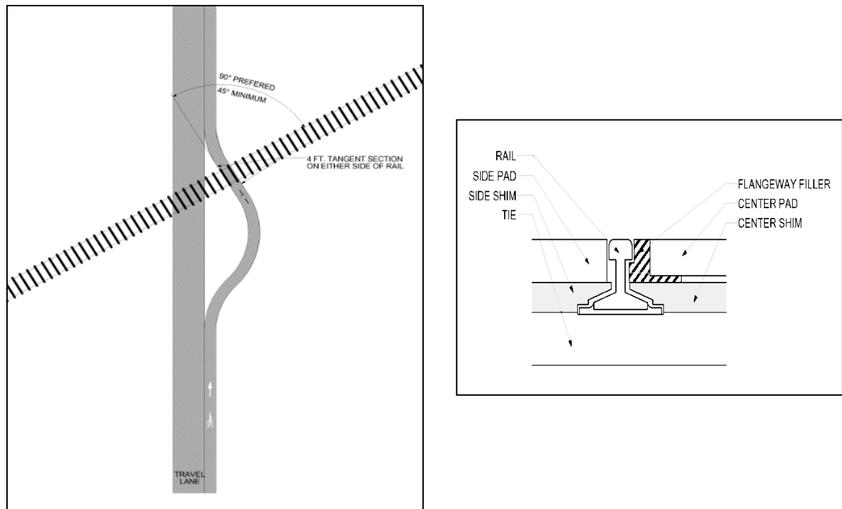
Figure: Angled Railroad Crossing
