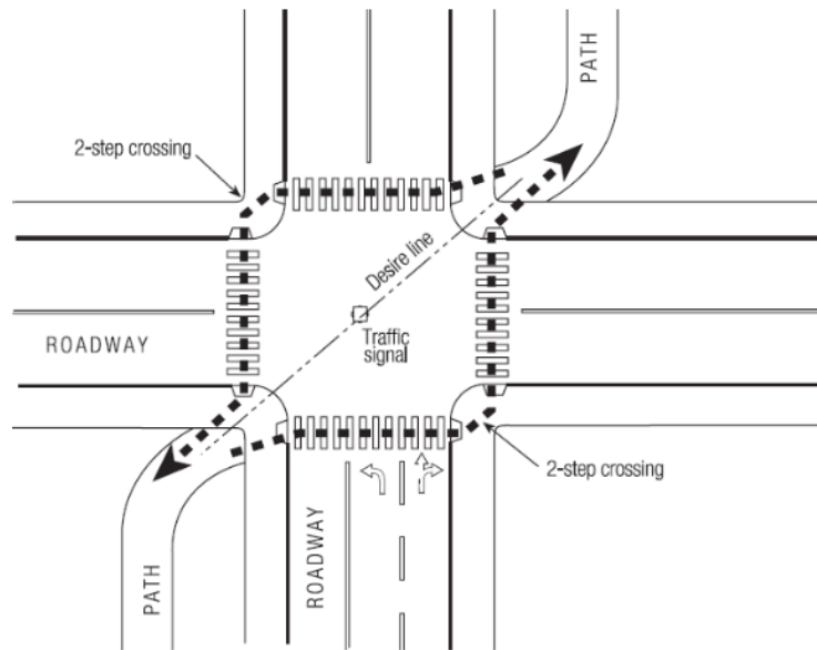
Figure: Two-Step Crossing
