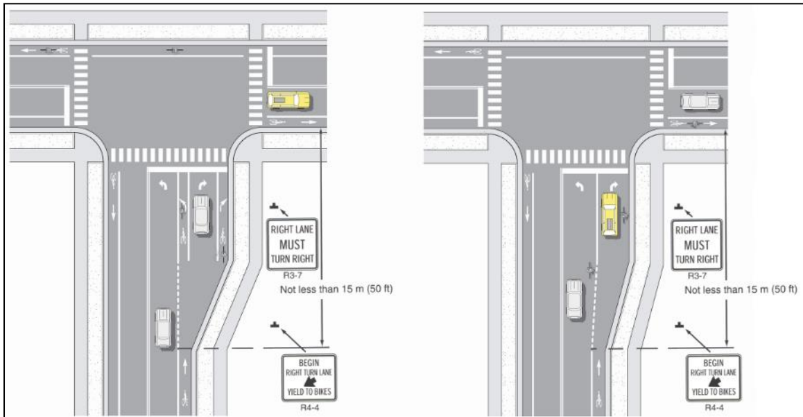
Figure: T-Intersections
