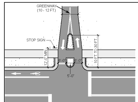
Figure: Motor Vehicle Barriers
