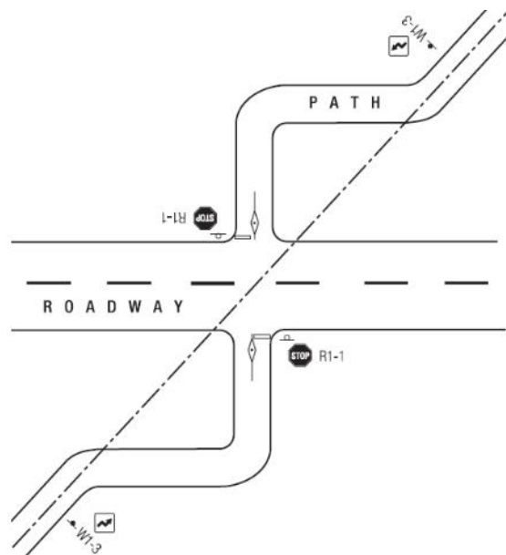
Figure: Ninety Degree Crossing
