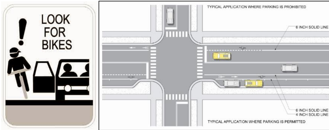
Figure: Adjacent to On-Street Parking
